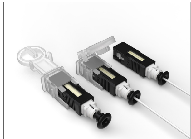
NPC+ (No Polish Connector) SC OM2, 250/900 μm including one semi-tight buffer clamp
