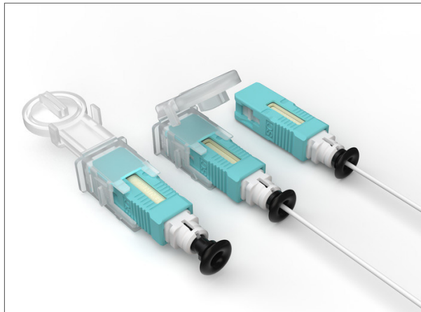
NPC+ (No Polish Connector) SC OM3/4, 250/900 \mu\text{m} including one semi-tight buffer clamp
