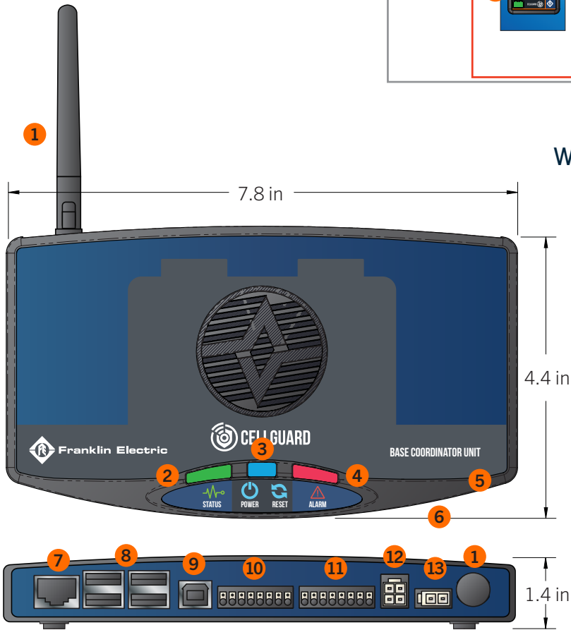
BASE COORDINATOR UNIT (BCU)
